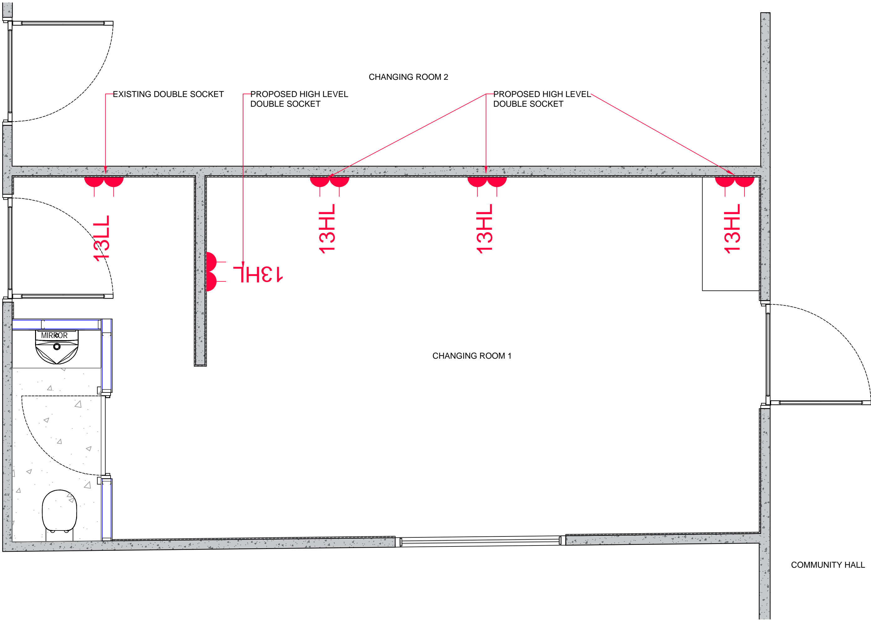
1 PROPOSED ELECTRICAL LAYOUT Scale: 1:25 @ A1 1:50 @A3
