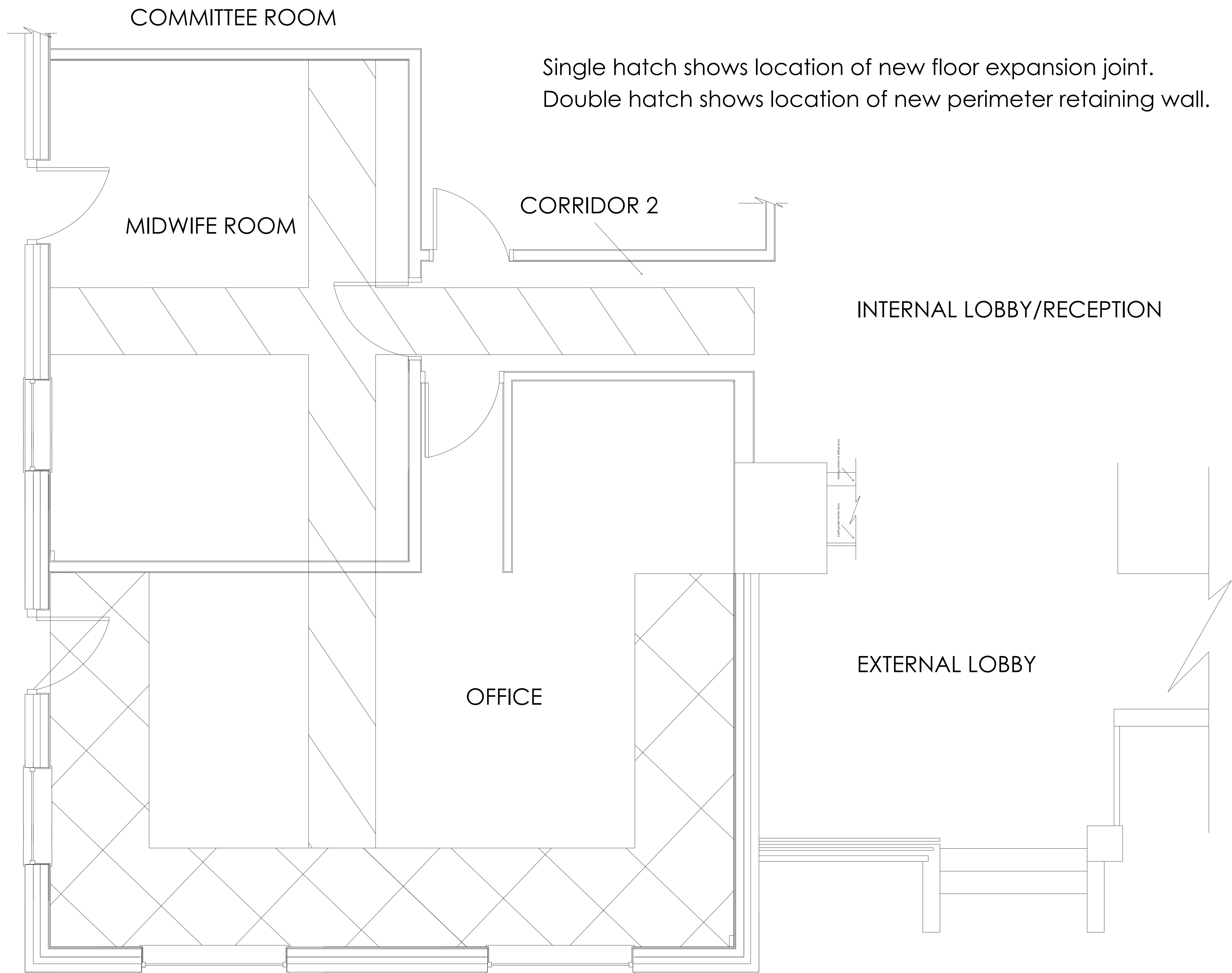
PROPOSED GF PLAN [LOCATION OF WORKS TO FLOOR] 1 OF 2 - DRAWING HAR021
