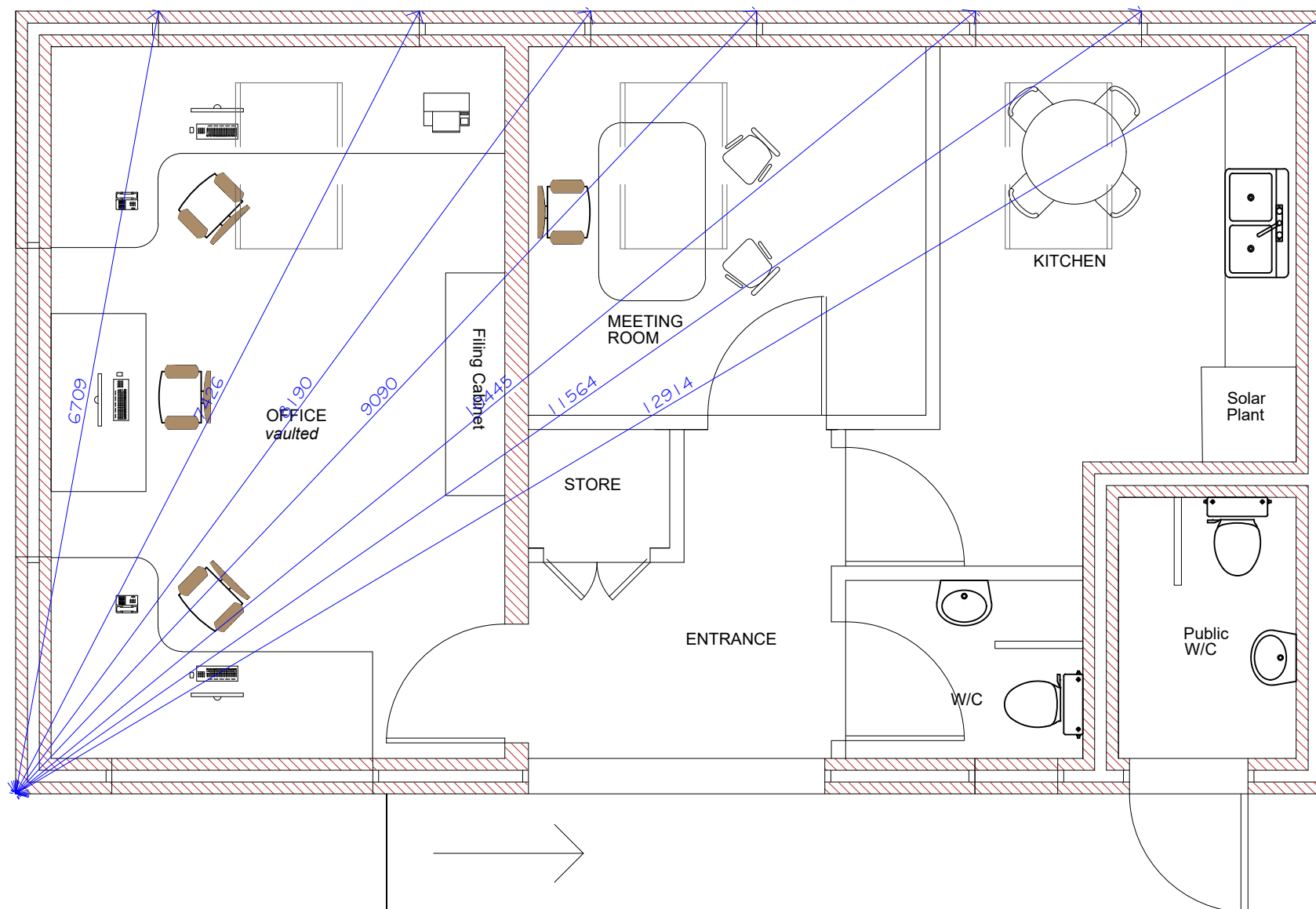
BRICKWORK DIAGONALS 1
