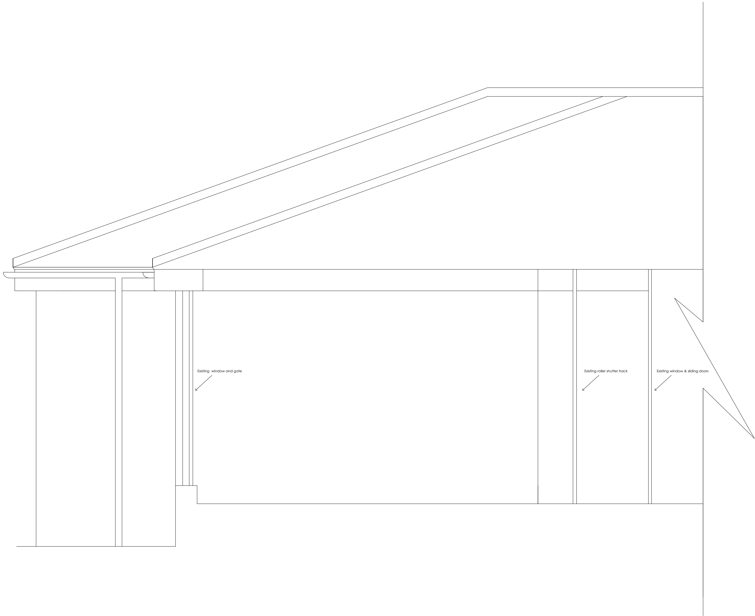
EXISTING RIGHT [WESTERN] ELEVATION - OFFICE - DRAWING HAR005
