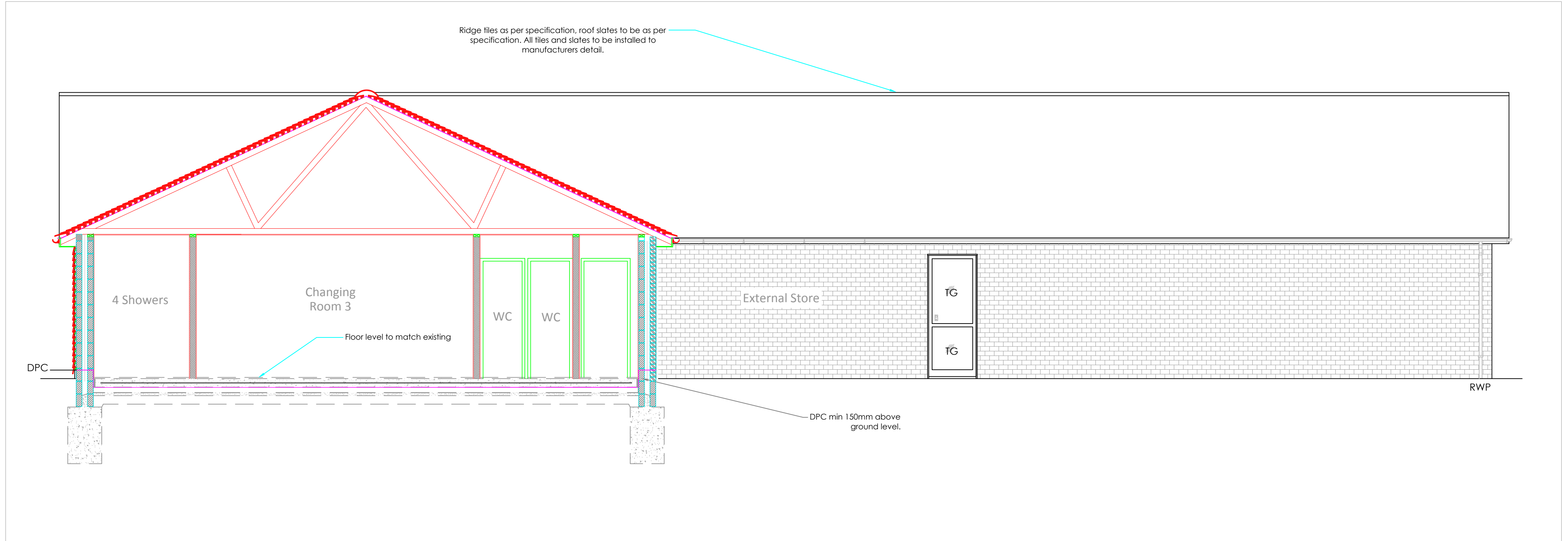
Proposed Section A-A 1:50 Scale
