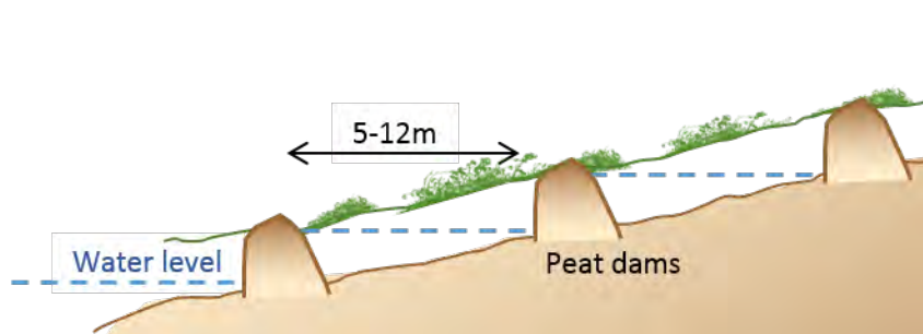
Figure 2 Dams showing top to toe spacing
