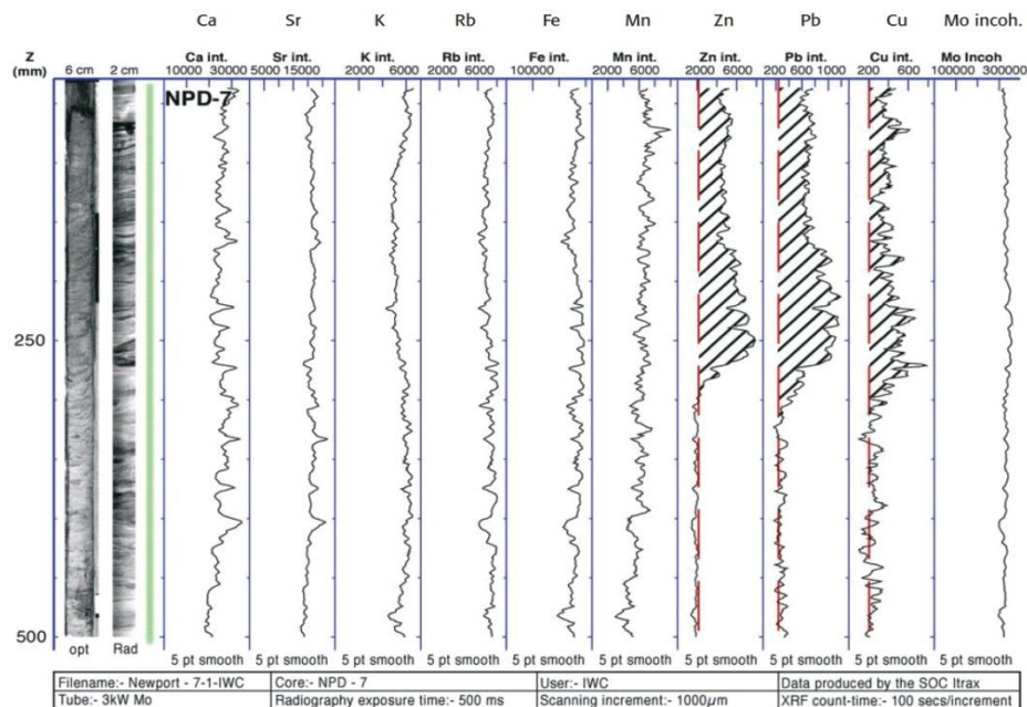
Figure 2: ITRAX optical, radiographic and element profiles for Newport Deep (Severn Estuary). The diagonal ornament highlights the zone of anthropogenic heavy metal pollution. The Molybdenum incoherent radiation (Compton scatter radiation) is a good indicator of mean atomic number and is used to assess matrix variations (courtesy Prof. I.W. Croudace, University of Southampton).
