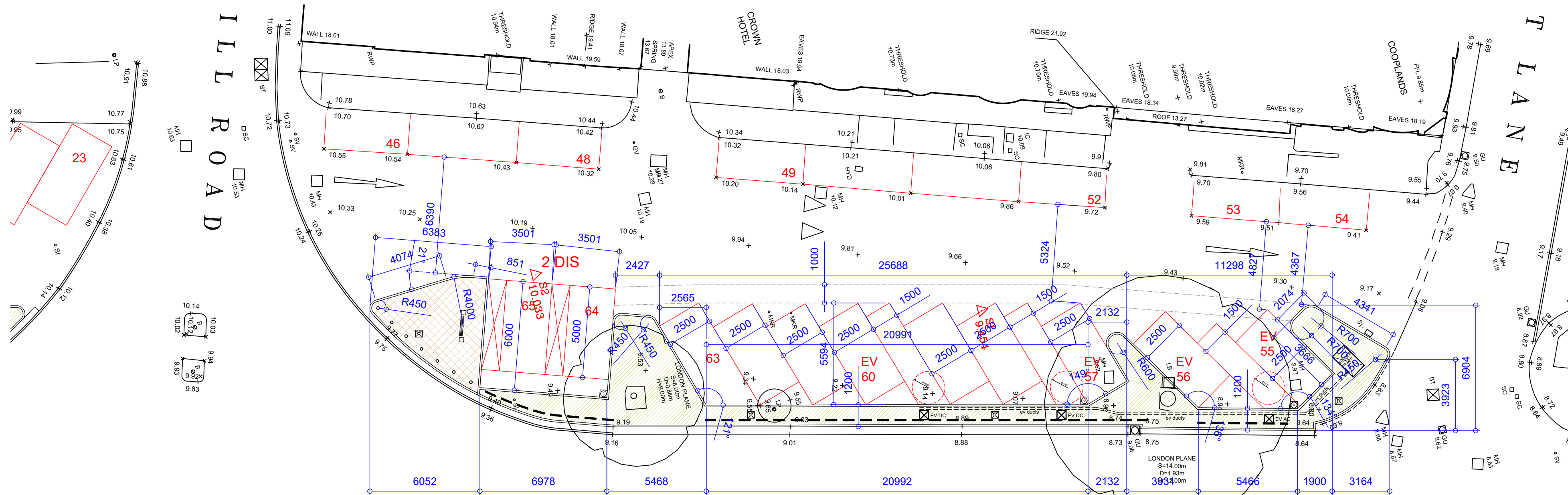
P 002 PARKING SET OUT SCALE 1-150 @ A1
