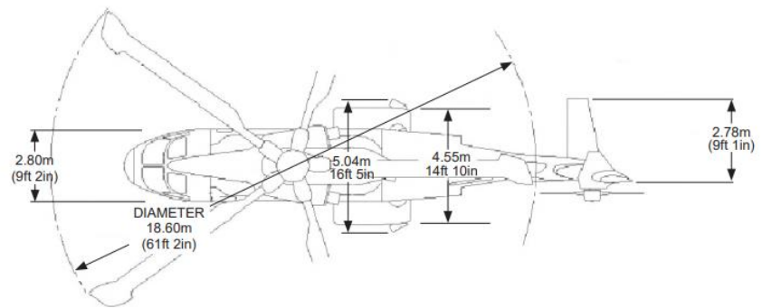
Overall Dimensions - Merlin HC (Mk4/4A)
