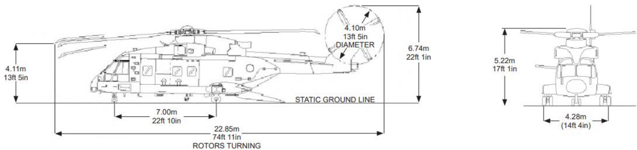
External Dimensions - Spread
