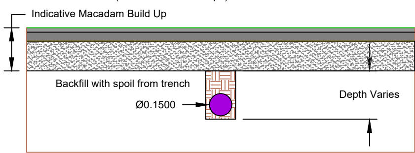
150mm Ø Main Drain (Solid Twin-walled Pipe) - Beneath Porous Macadam Road
