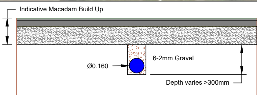
160mm Ø Collector (Perforated Plastic Pipe) - Beneath Porous Macadam Road/Path
