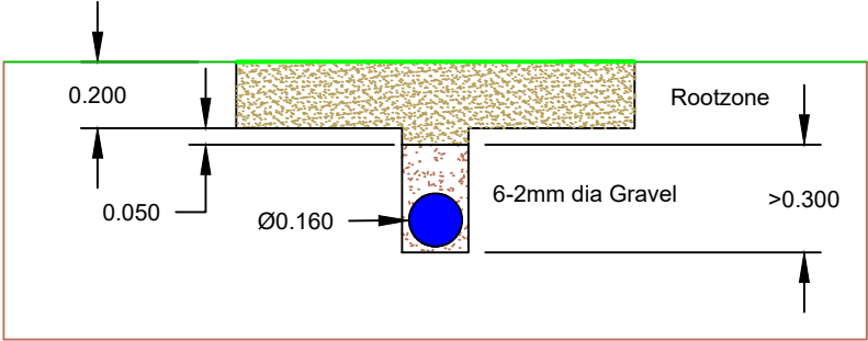
160mm Ø Collector (Perforated Plastic Pipe) - Beneath Grass Paths
