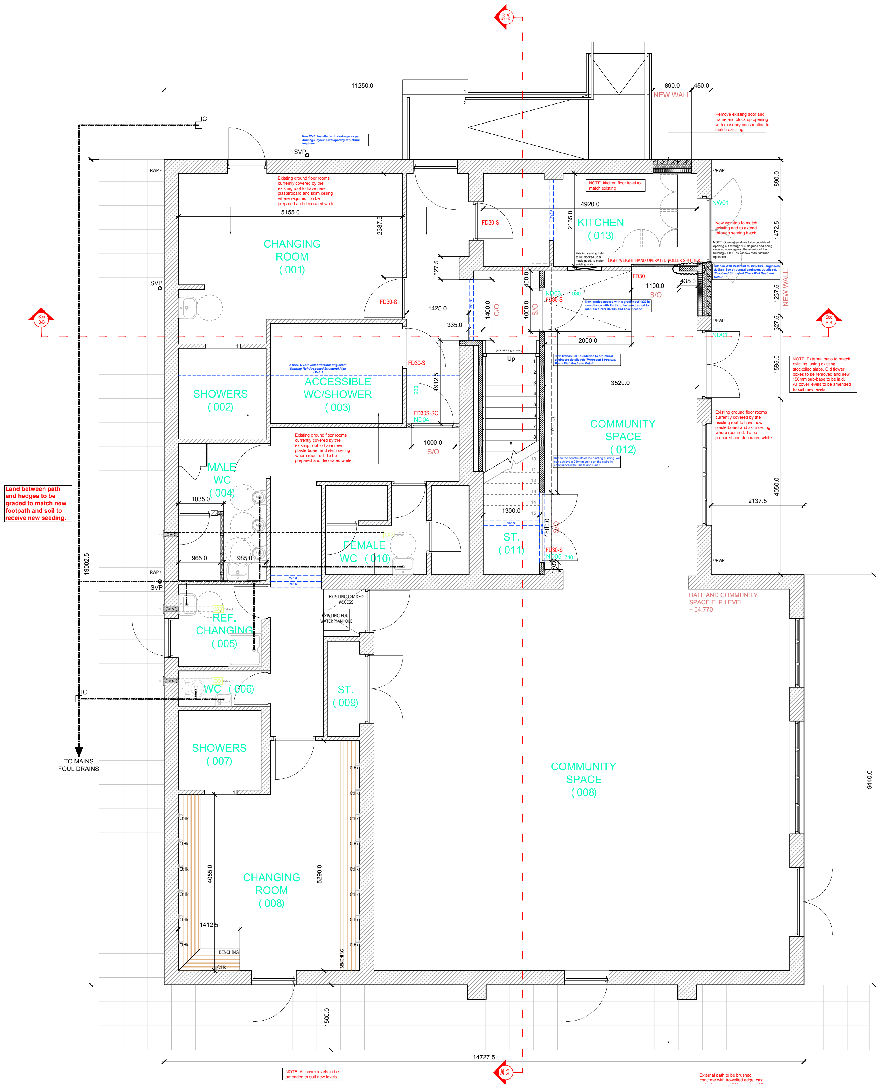
GROUND FLOOR PLAN, SCALE: 1:50 @ A1
