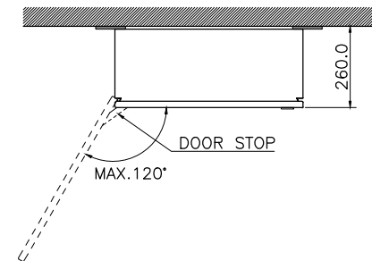
BOTTOM VIEW (SCALE 1:10)
