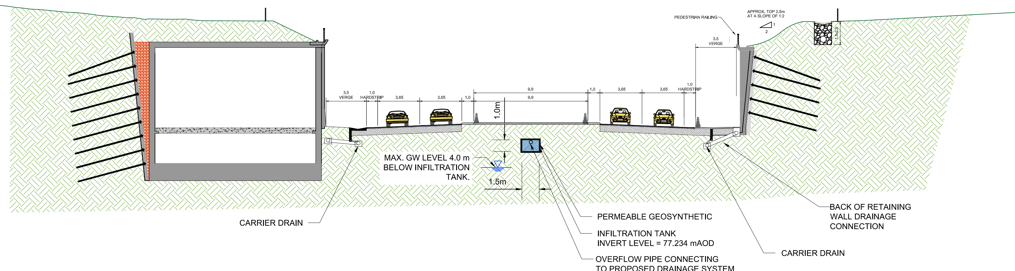
SECTION A-A Chainage 10550.000
