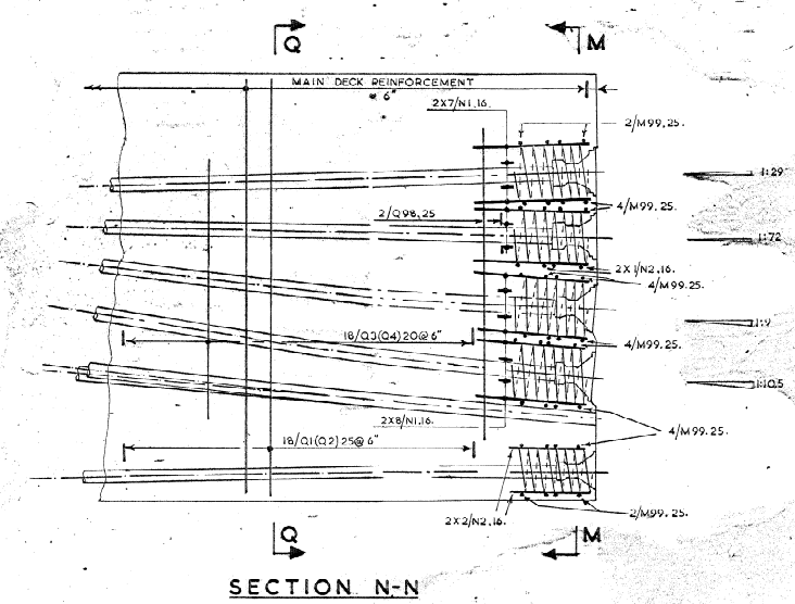
TYPICAL DETAILS OF ANCHORAGES AND COUPLERS AT END OF CANTILEVER
