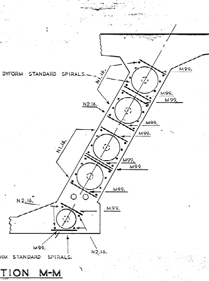
TYPICAL DETAILS OF ANCHORAGES AND COUPLERS AT END OF CANTILEVER
