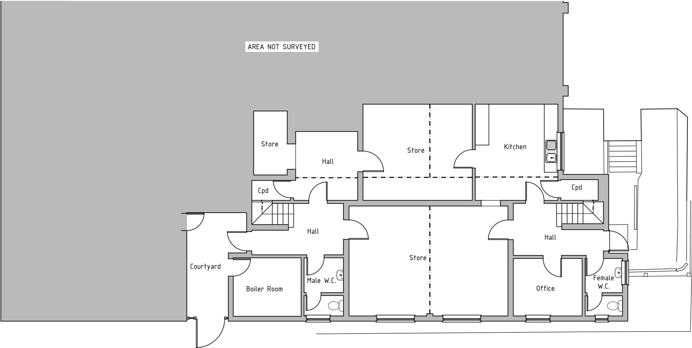
Existing Lower Ground Floor Plan 1:100
