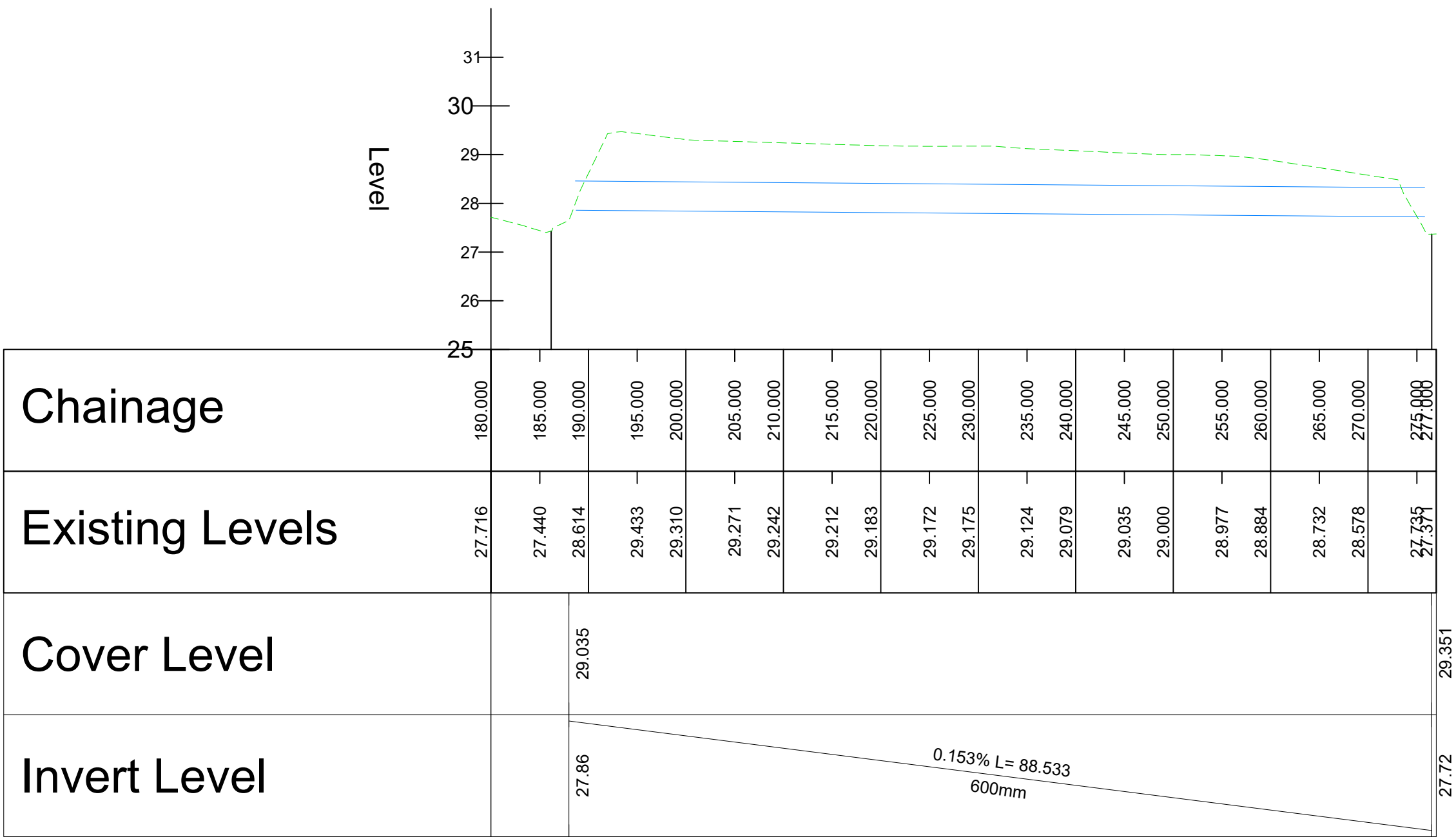
PIPE ALIGNMENT - LONGSECTION CHG. 180-277 SCALE: H 1:500,V 1:100. DATUM: 25.000
