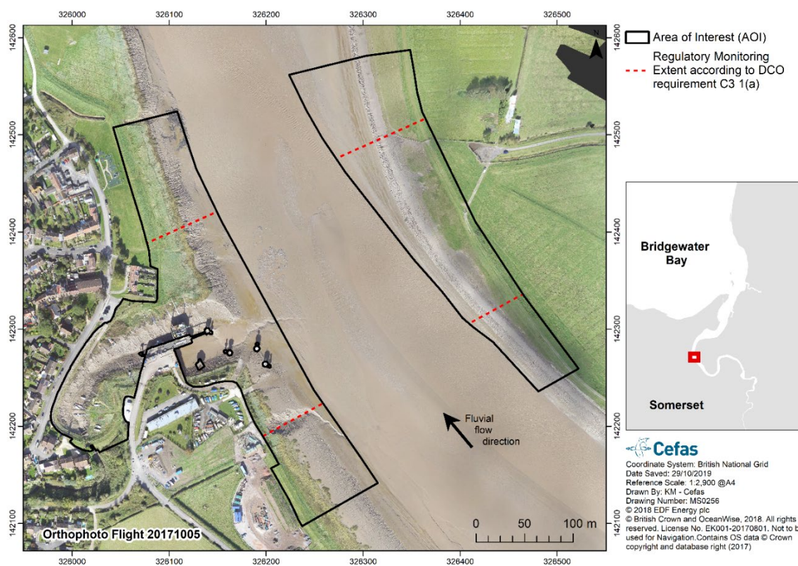
Figure 2: The survey area at Combwich. Ground control point and ground control point markers are required in the area of interest (AOI). Full details of the flight areas are supplied as part of the tender package.
