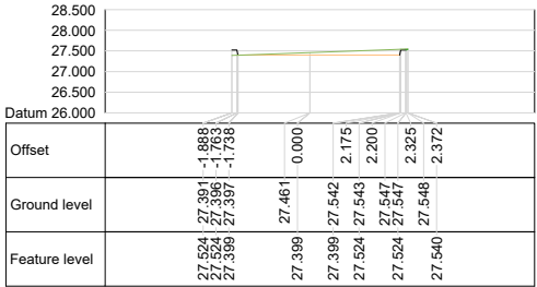
Alignment ACCESS ROAD Chainage 40.000
