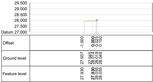
Alignment ACCESS ROAD Chainage 91.345
