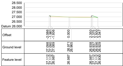
Alignment ACCESS ROAD Chainage 25.000
