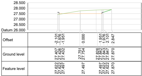
Alignment ACCESS ROAD Chainage 50.000
