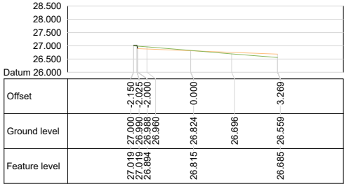
Alignment ACCESS ROAD Chainage 10.000
