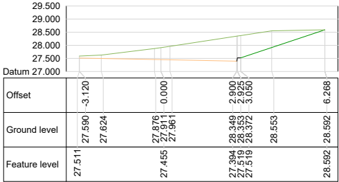
Alignment ACCESS ROAD Chainage 70.000
