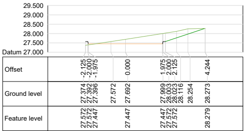
Alignment ACCESS ROAD Chainage 55.000
