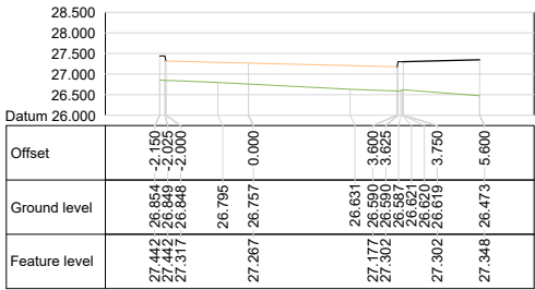
Alignment ACCESS ROAD Chainage 0.000
