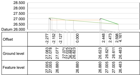
Alignment ACCESS ROAD Chainage 20.000
