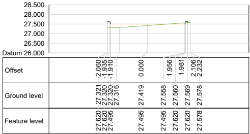
Alignment ACCESS ROAD Chainage 45.000
