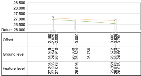
Alignment ACCESS ROAD Chainage 5.000
