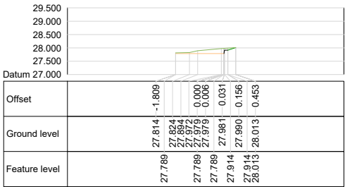
Alignment ACCESS ROAD Chainage 85.000
