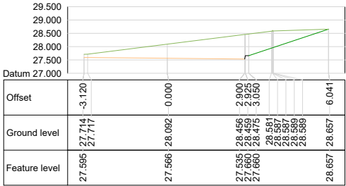
Alignment ACCESS ROAD Chainage 75.000
