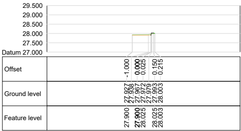
Alignment ACCESS ROAD Chainage 90.000
