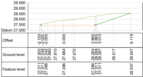
Alignment ACCESS ROAD Chainage 65.000
