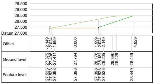
Alignment ACCESS ROAD Chainage 60.000
