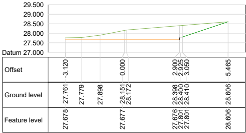
Alignment ACCESS ROAD Chainage 80.000
