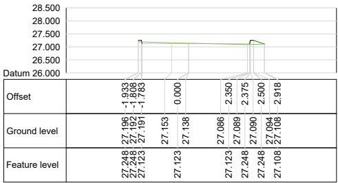
Alignment ACCESS ROAD Chainage 30.000
