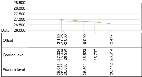
Alignment ACCESS ROAD Chainage 15.000
