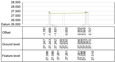
Alignment ACCESS ROAD Chainage 35.000
