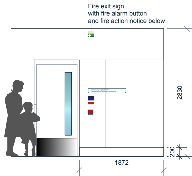
ENTRANCE ELEVATION 1:50
