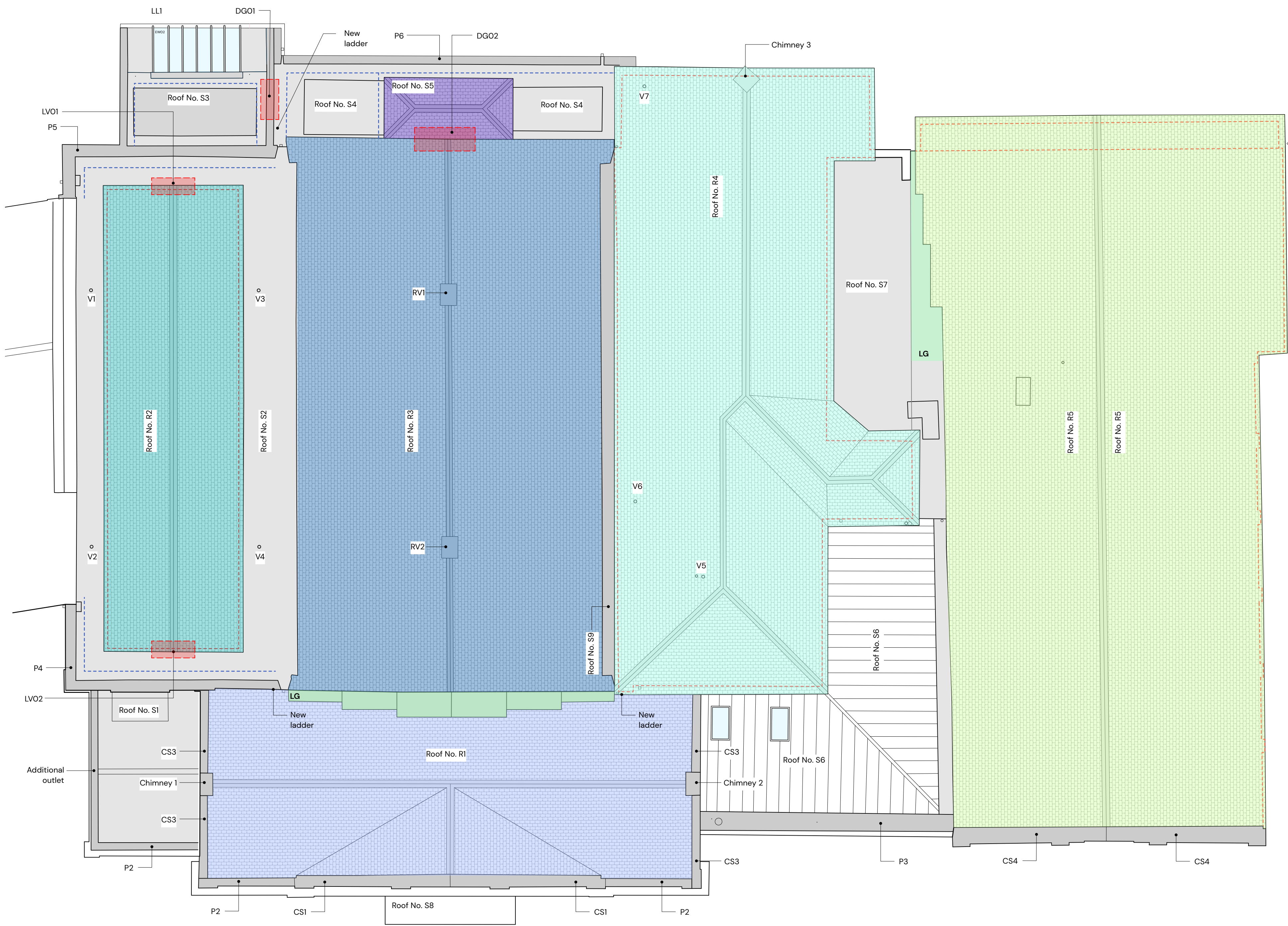
Proposed Pitched Roof Plan
