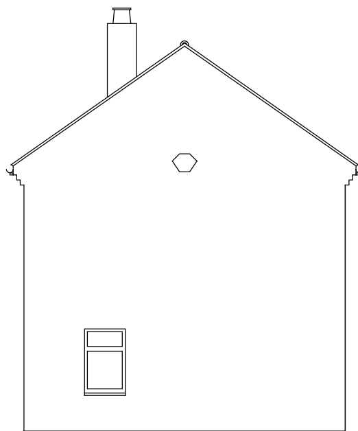
01 NORTH ELEVATION - AS EXISTING 1200 1:100 @ A3
