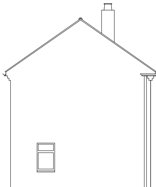
03 SOUTH ELEVATION - AS EXISTING 1200 1:100 @ A3
