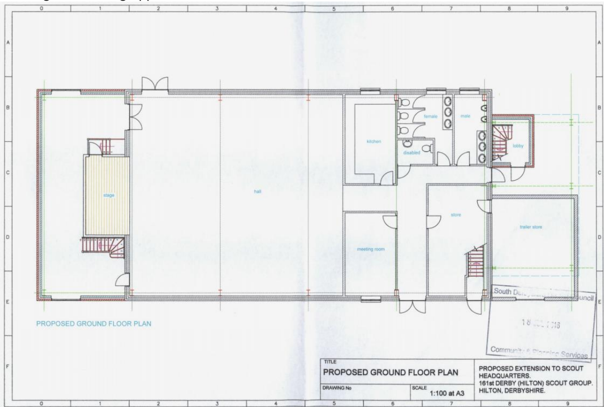
Drawing 3 – Planning Application Ground Floor
