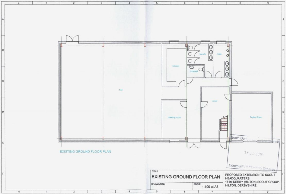
Drawing 1 – Existing Ground Floor
