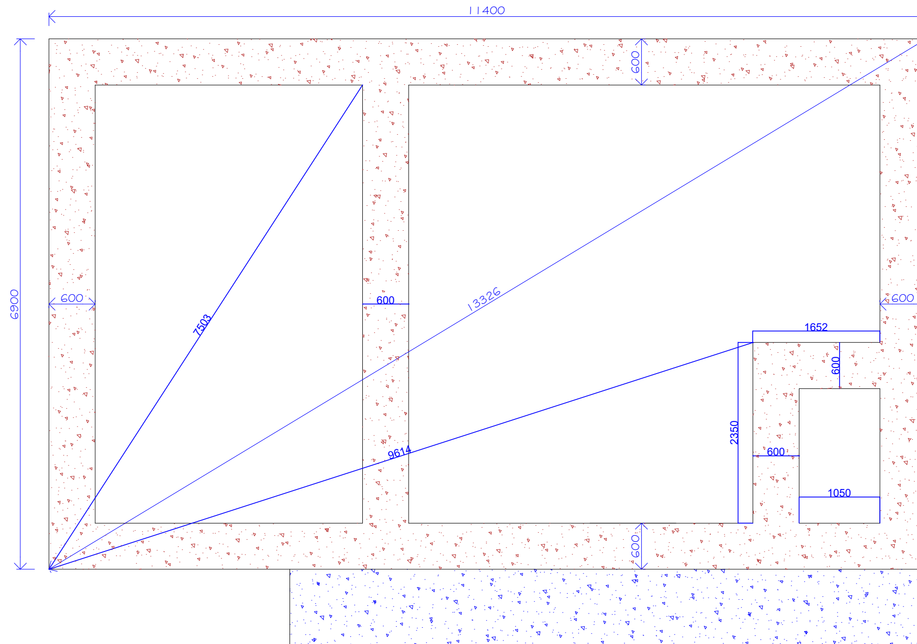
FOUNDATION SETTING-OUT
