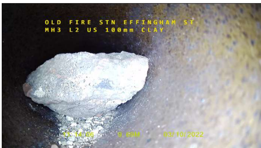
Photo: 13_13_91_A.jpg 9.09m, Settled deposits, coarse, 50% cross-sectional area loss
