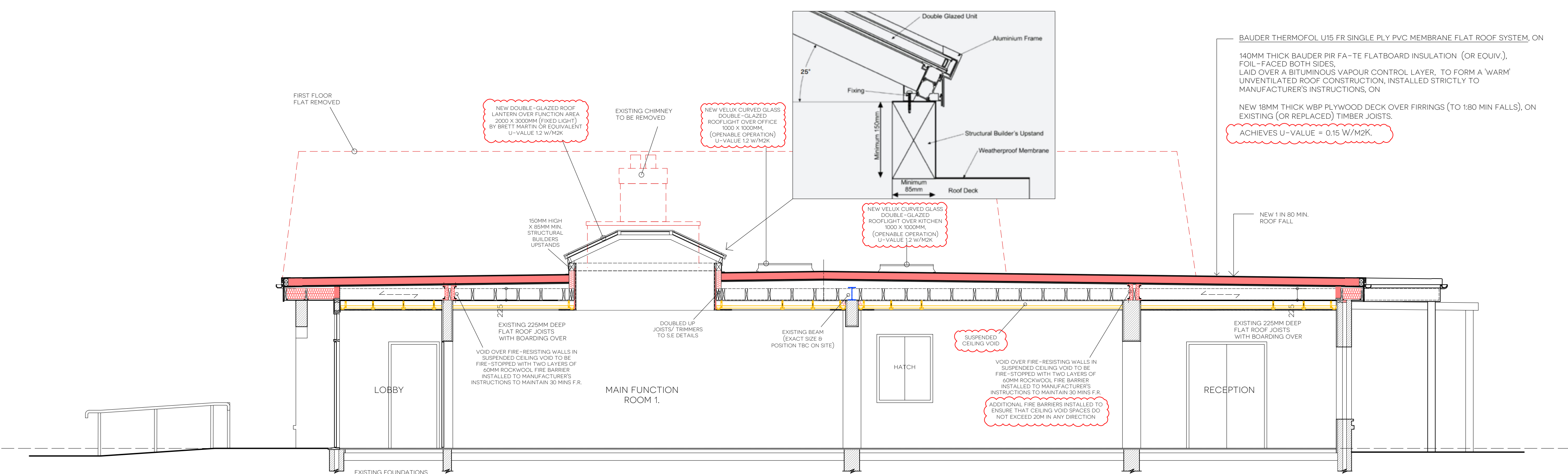
PROPOSED SECTION B-B SCALE: 1:50 @ A1
