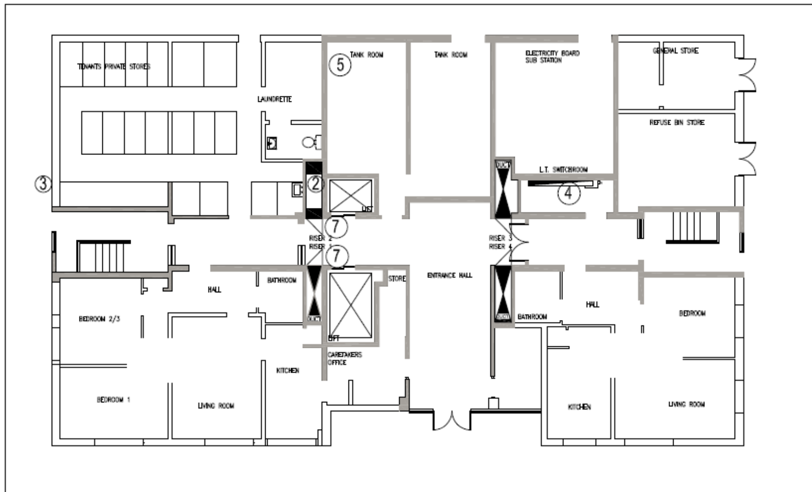
STOREY FLAT GROUND FLOOR LAYOUT
