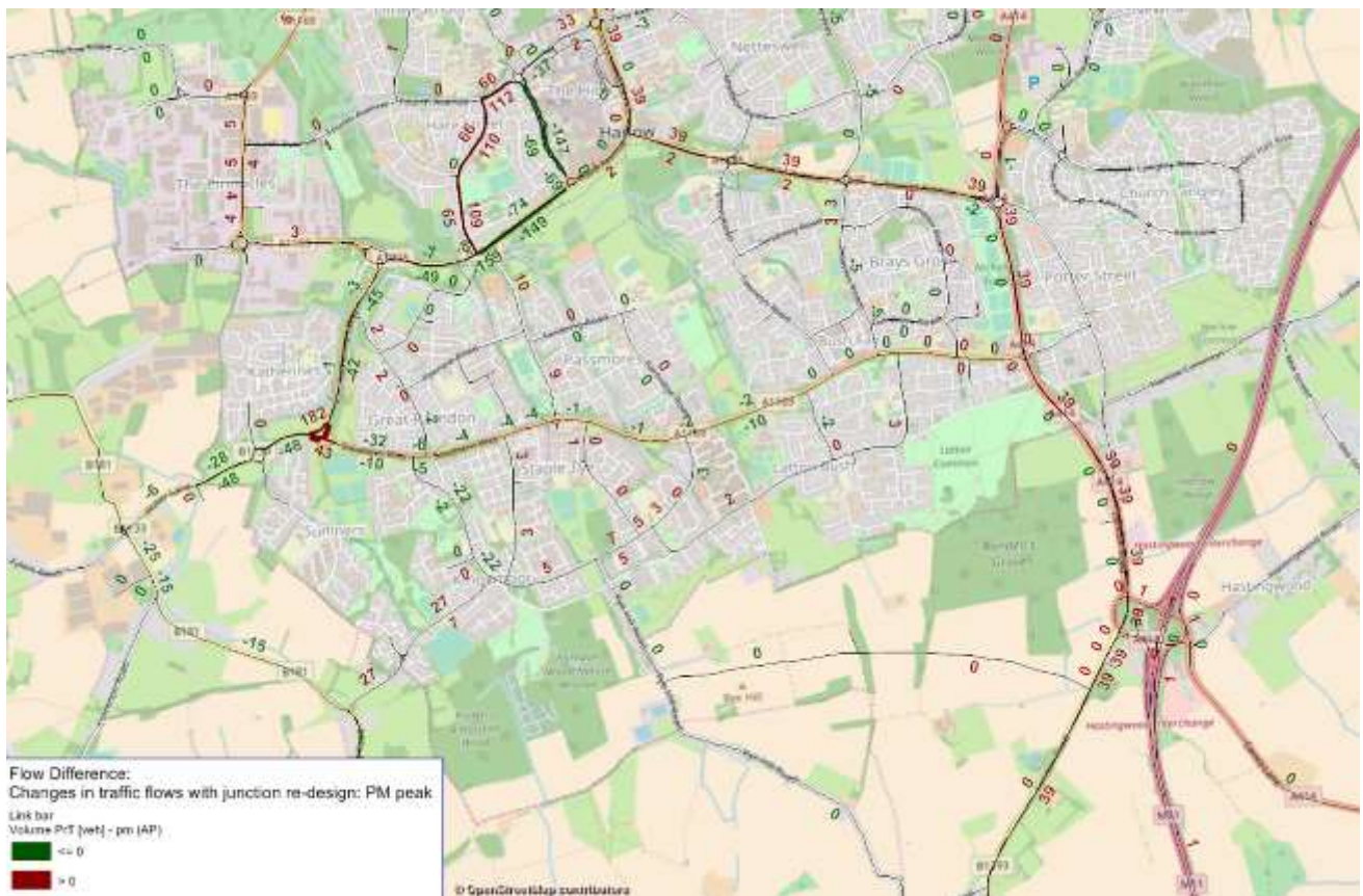
Figure 5-16 - Changes in Wider Harlow Development Traffic Flow with Junction Re-Design – PM Peak Hour
