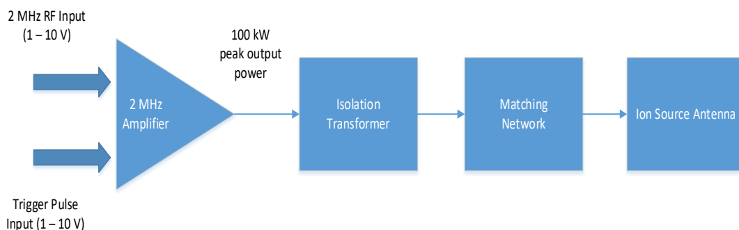
Figure 1: Block diagram of amplifier connected to other equipment in the ion source
