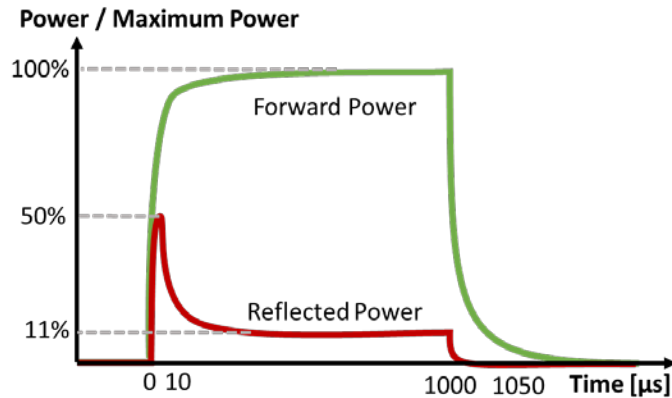
Figure 2: Expected forward and reflected power envelopes, highlighting the need to withstand high reflected power at the start of each RF pulse.
