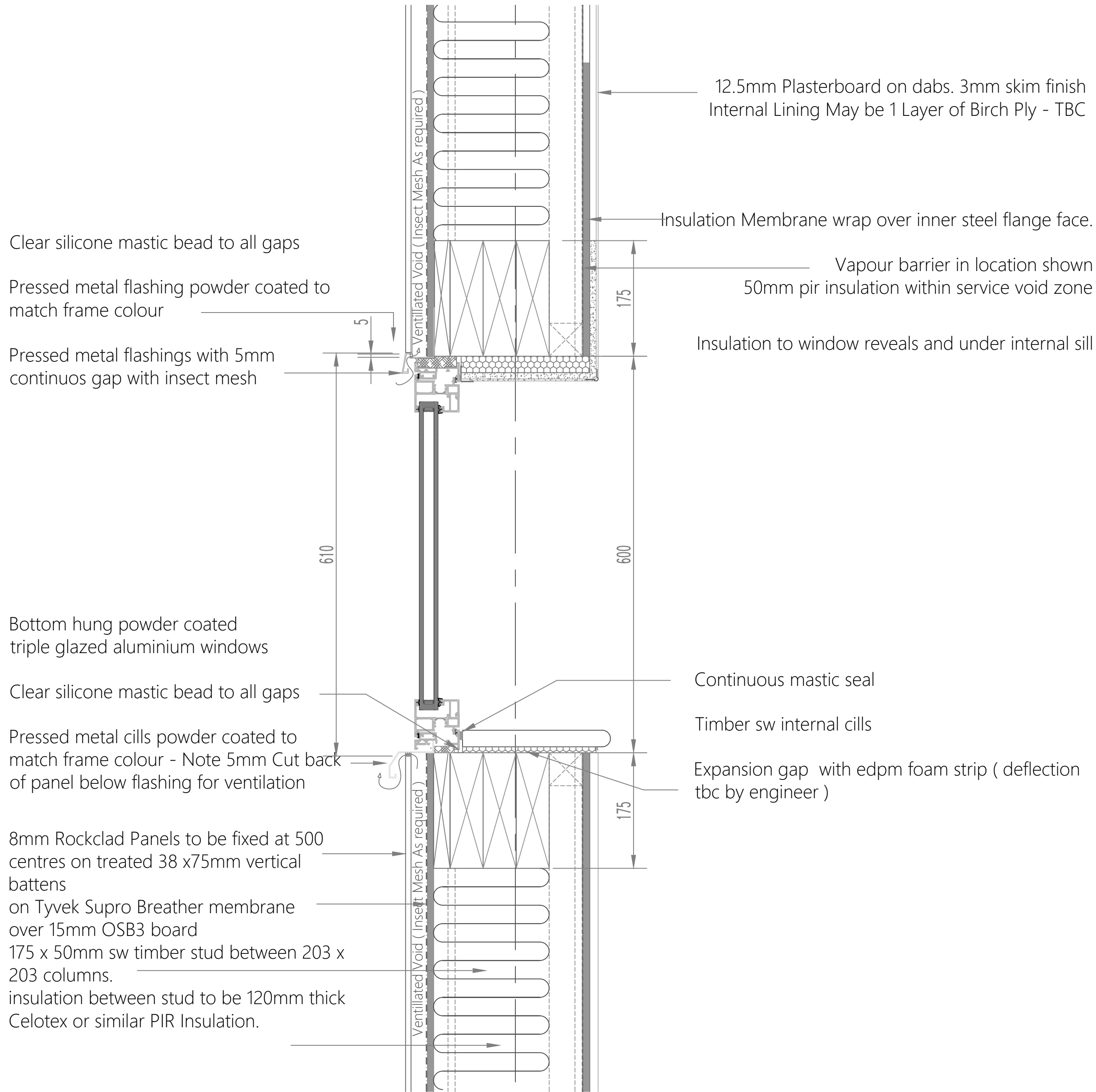
Typical Head And Cill Detail 600h Windows to Gridline 1 Shown.
