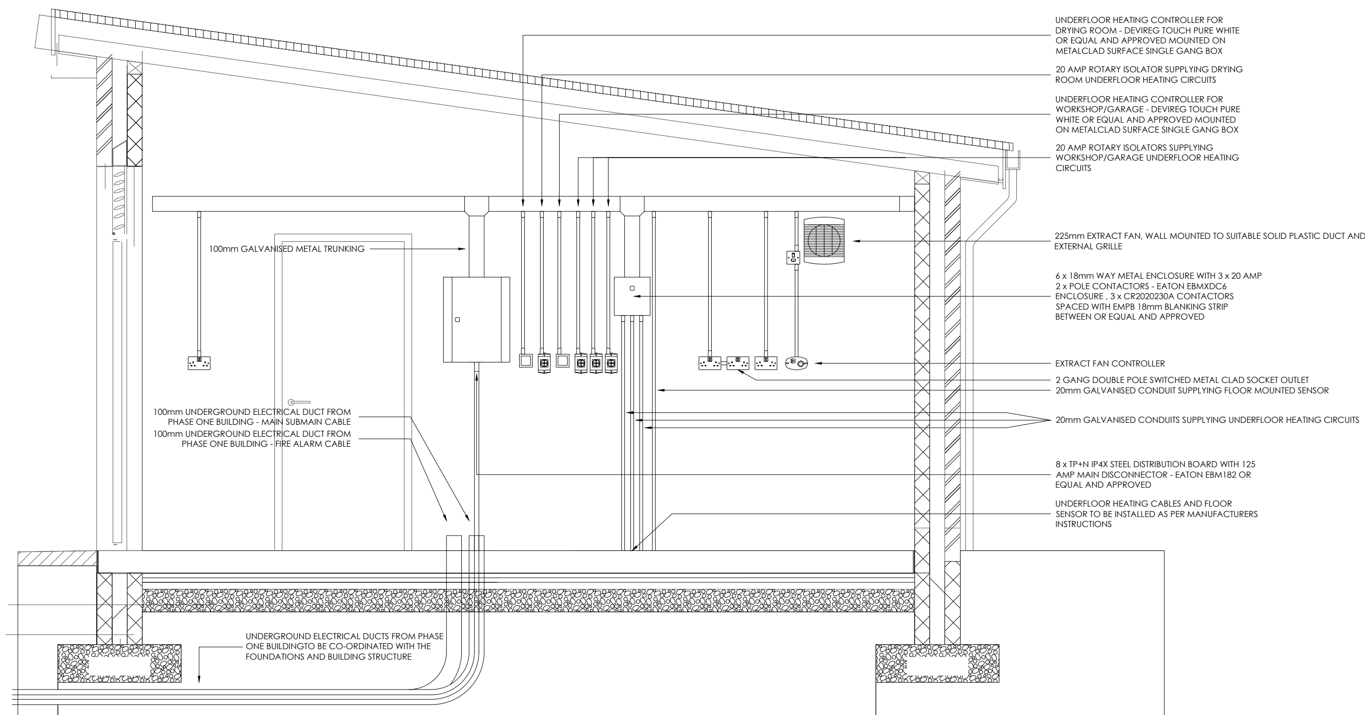
2 PROPOSED WORKSHOP/GARAGE ELECTRICAL DISTRIBUTION WALL DETAIL Scale : 1:25
