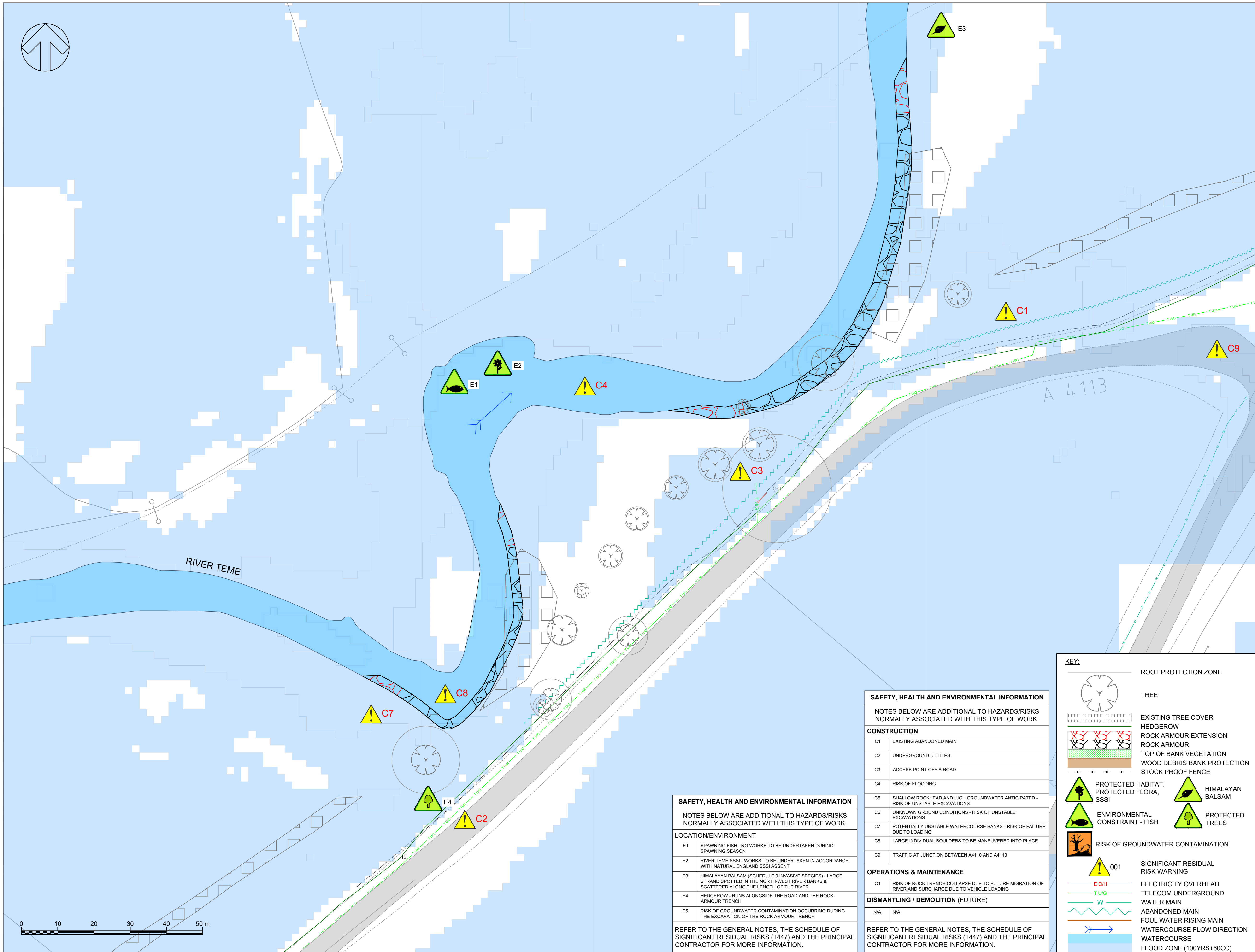
HAZARD PLAN SCALE 1: 500 @ A1 SCALE 1: 1000 @ A3
