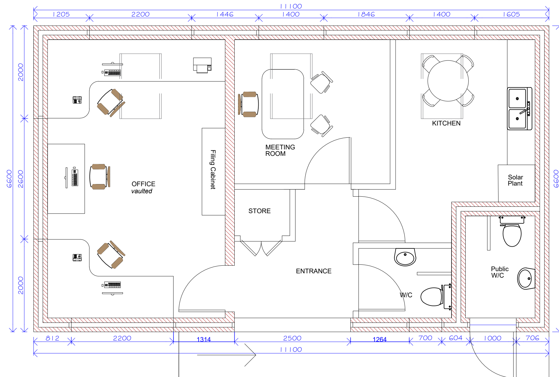
BRICKWORK SETTING-OUT
