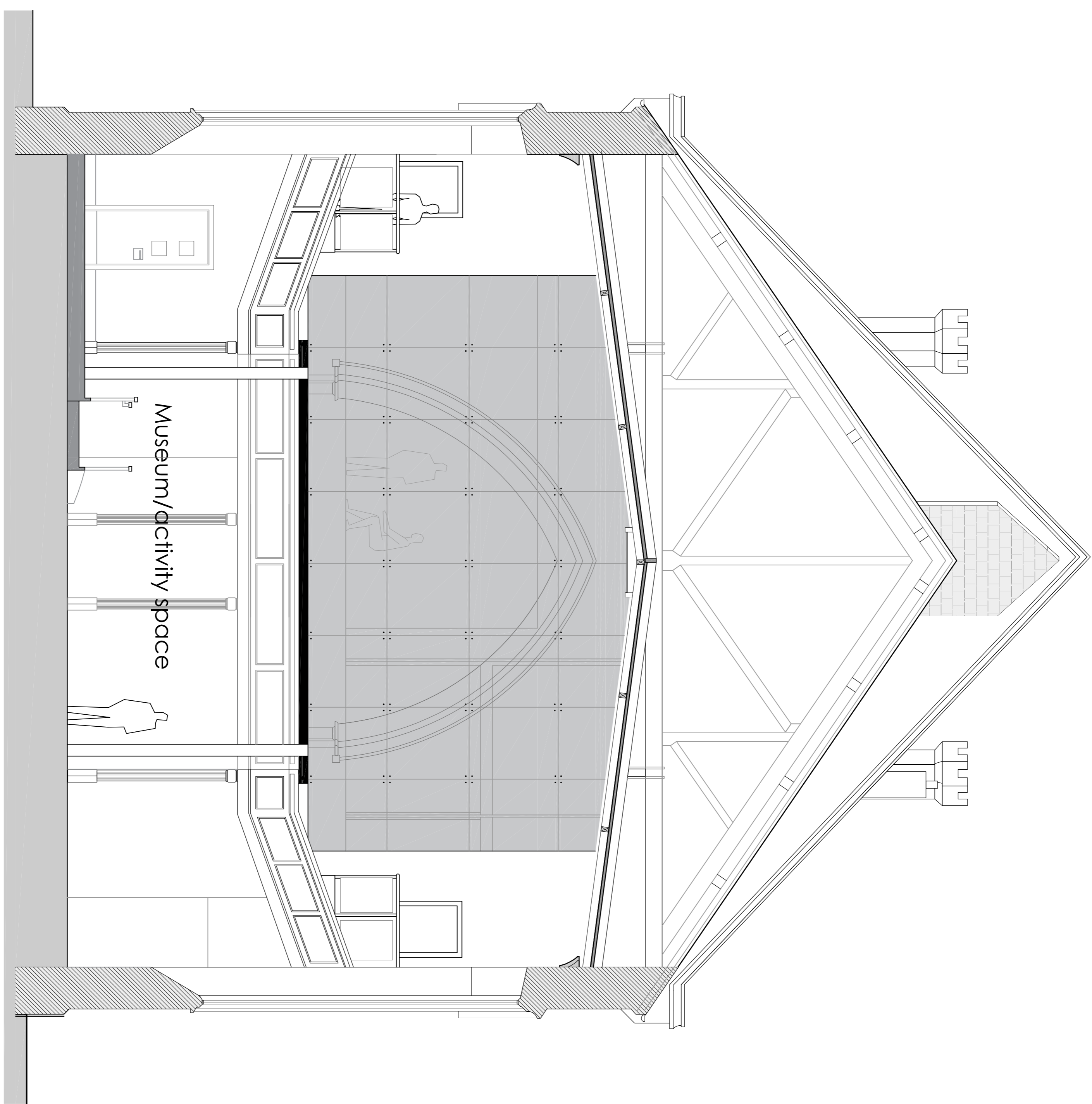
Section F-F
