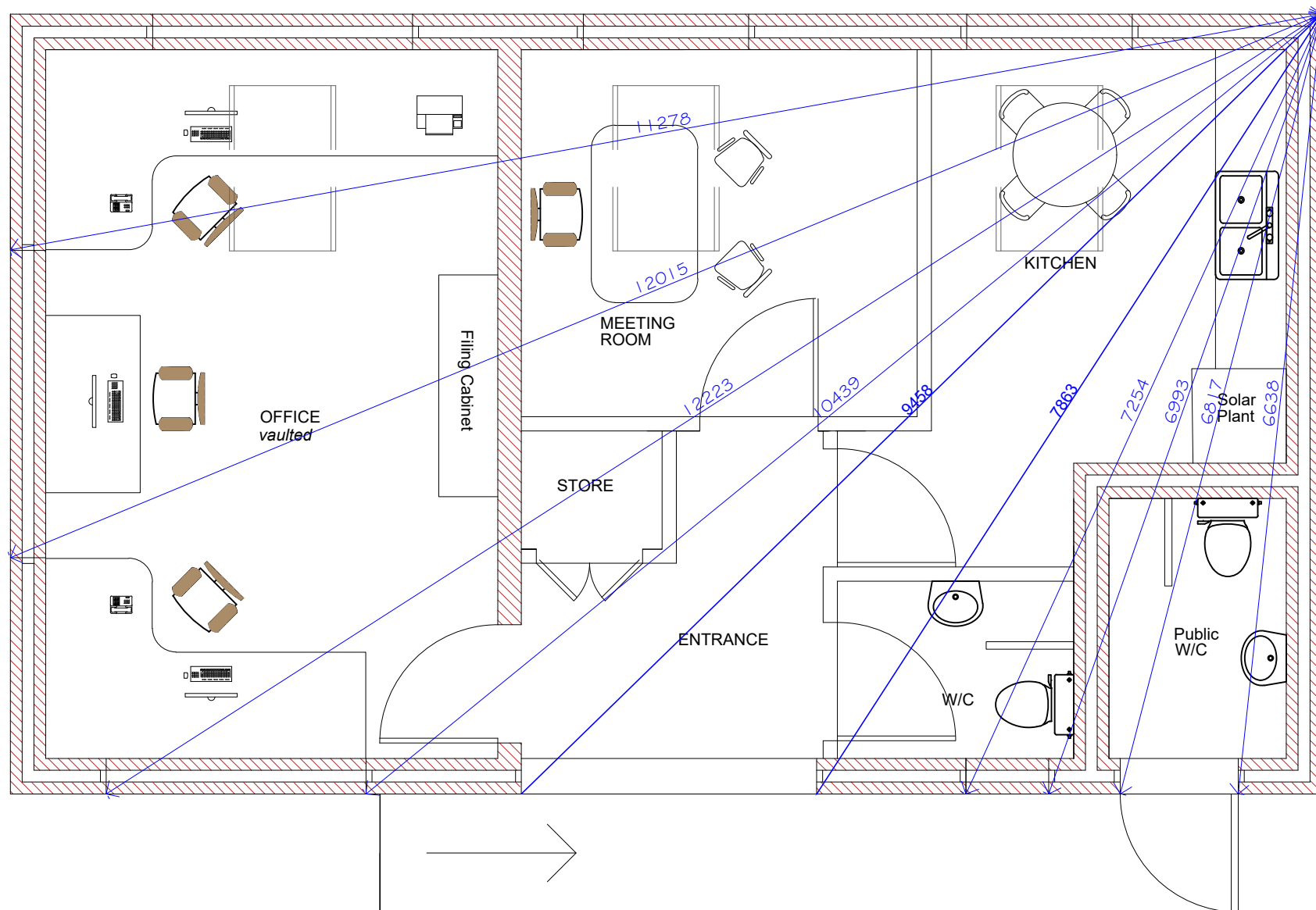
BRICKWORK DIAGONALS 2
