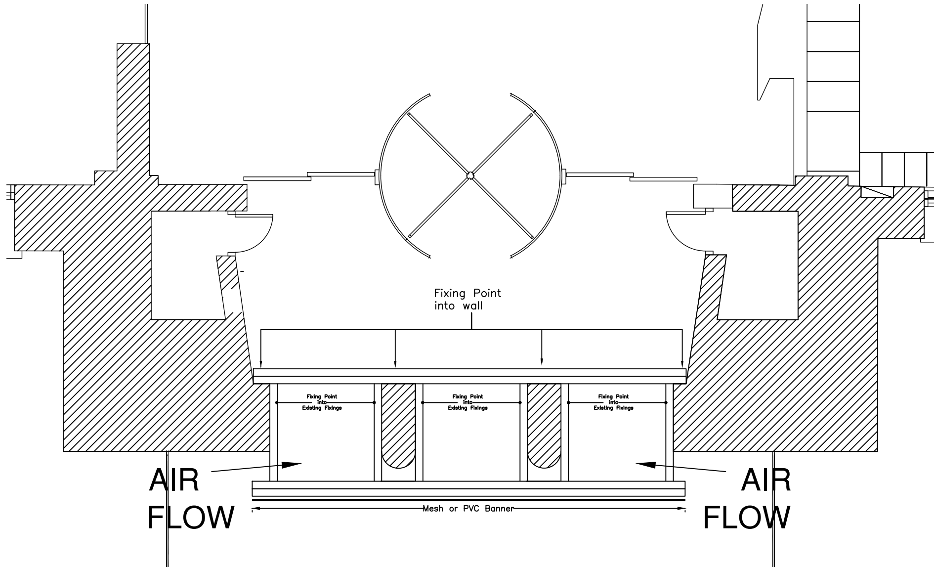
Plan View - Banner Details Scale 1/50 @ A3
