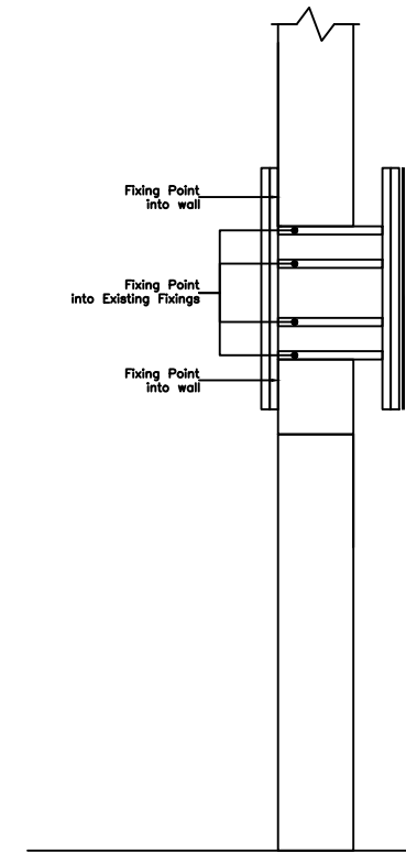
Section View - Banner Details Scale 1/100 @ A3
