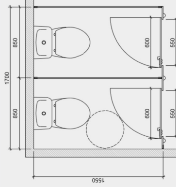
TYPICAL CORNER RANGE WC CUBICLES (without IPS Duct Panels)
