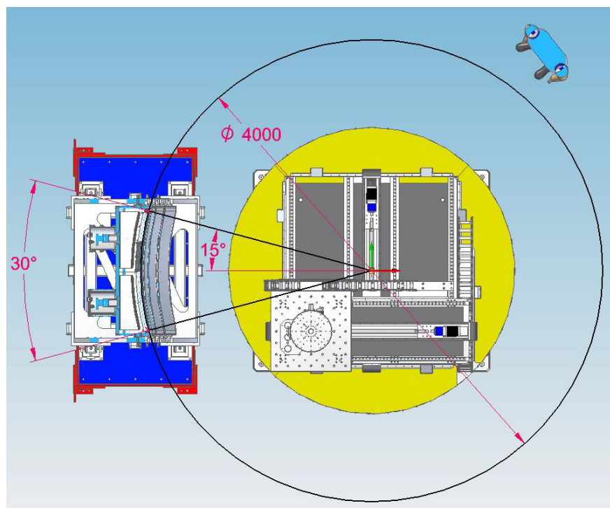
Figure 4 - Detector horizontal coverage
