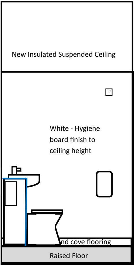
Area 6 - Staff/Visitor Toilet—Elevations
