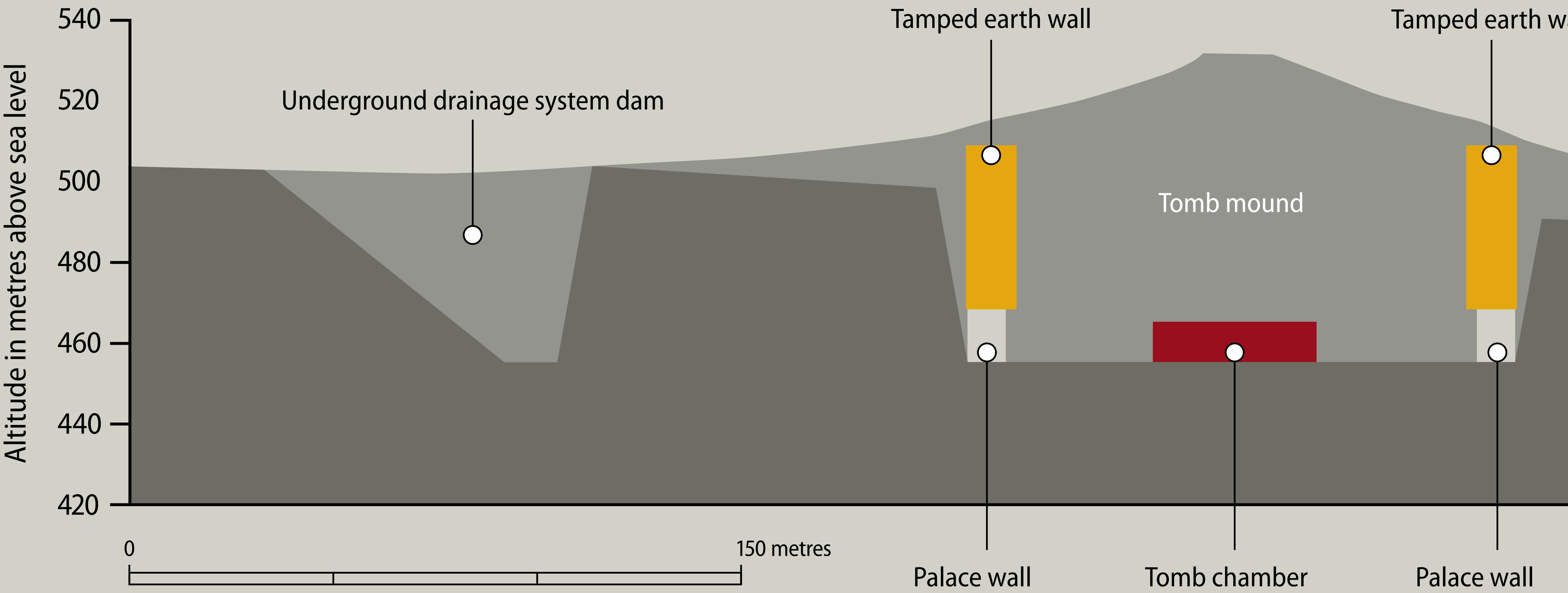
Cross-section of the tomb mound viewed westwards showing the underground palace and tomb chamber
