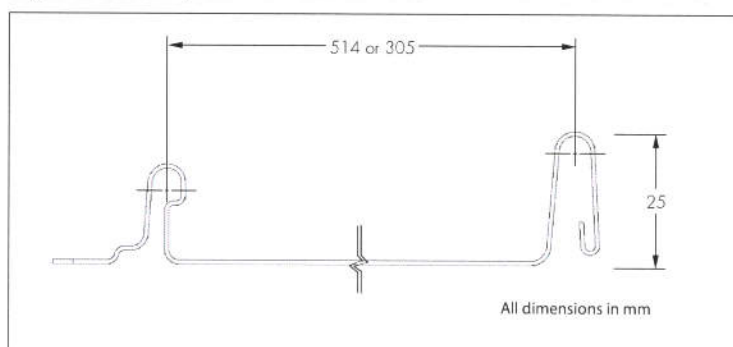
Figure 1 Panel profile
