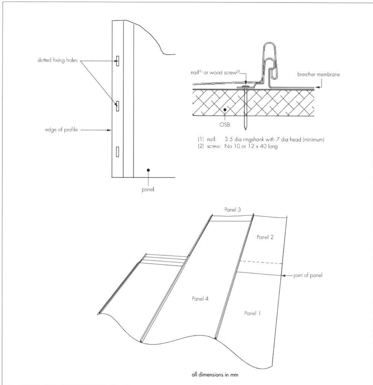
Figure 3 fixing details
