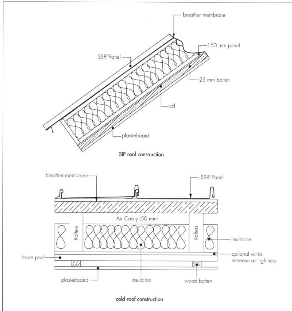
Figure 2 Typical installation
