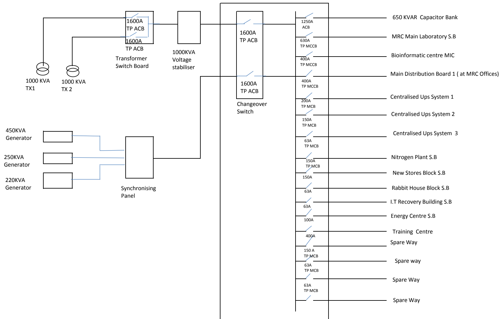
1600A ACB - Type TPN main low voltage Switch Board
