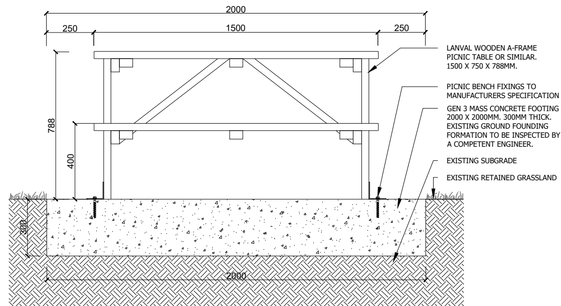
PICNIC BENCH WITH CONCRETE BASE - SIDE VIEW 1 - 1:20 @ A3
