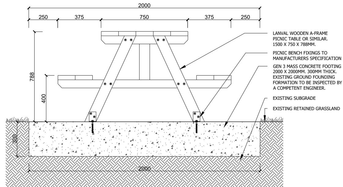
PICNIC BENCH WITH CONCRETE BASE - SIDE VIEW 2 - 1:20 @ A3
