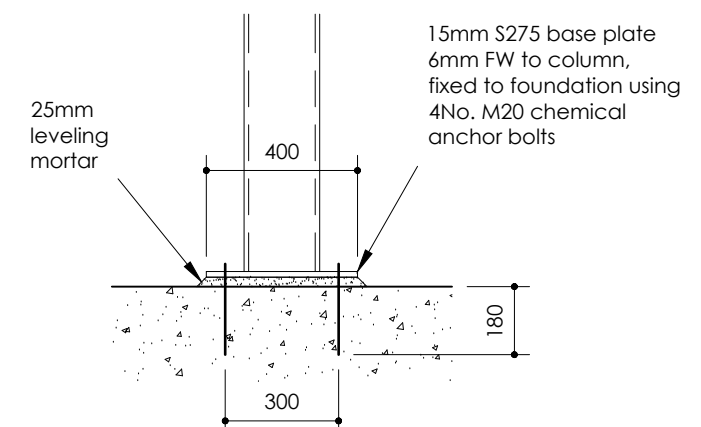
200 x 200 SHS BASEPLATE DETAIL (1/20)
