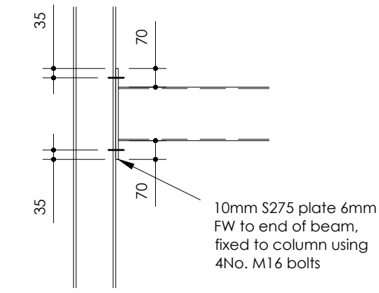
CONNECTION DETAIL 2 (1/20)
