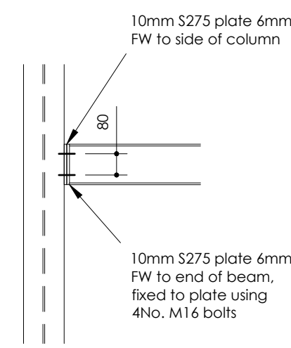
CONNECTION DETAIL 1 (1/20)
