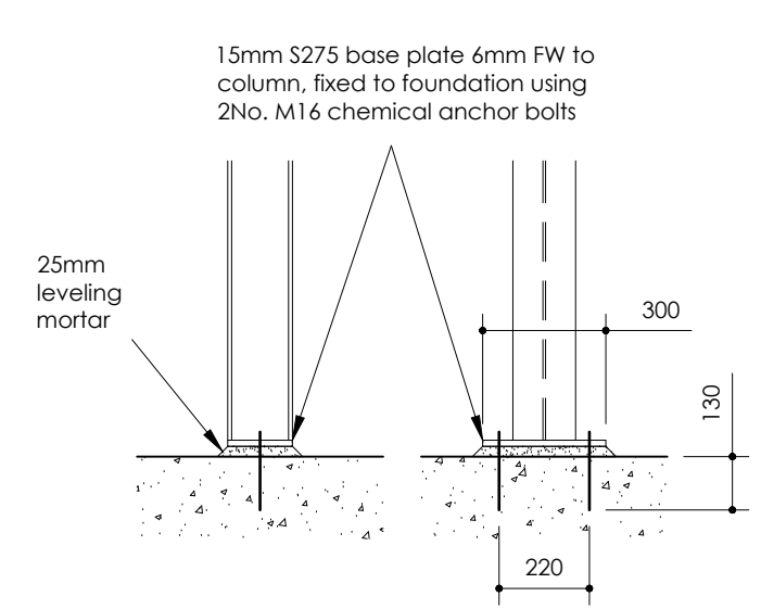
152 x 152 UC BASEPLATE DETAIL (1/20)
