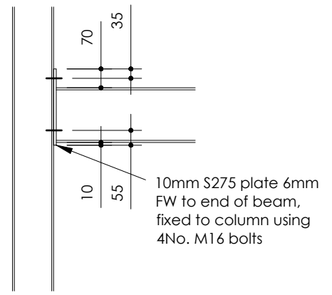
CONNECTION DETAIL 4 (1/20)
