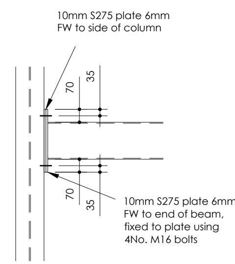
CONNECTION DETAIL 2 (1/20)
