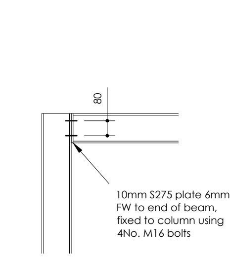
CONNECTION DETAIL 1 (1/20)
