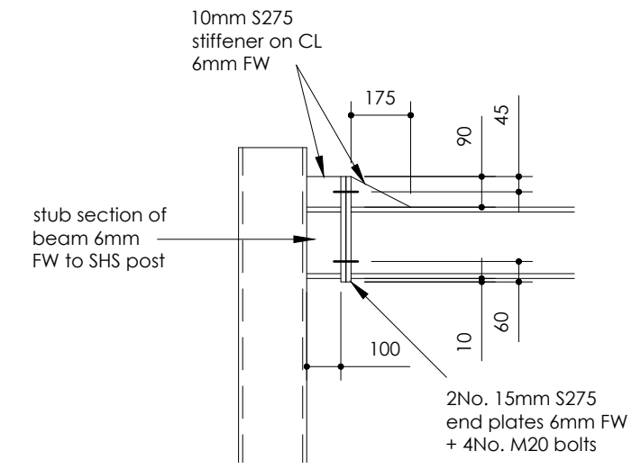
CONNECTION DETAIL 3 (1/20)
