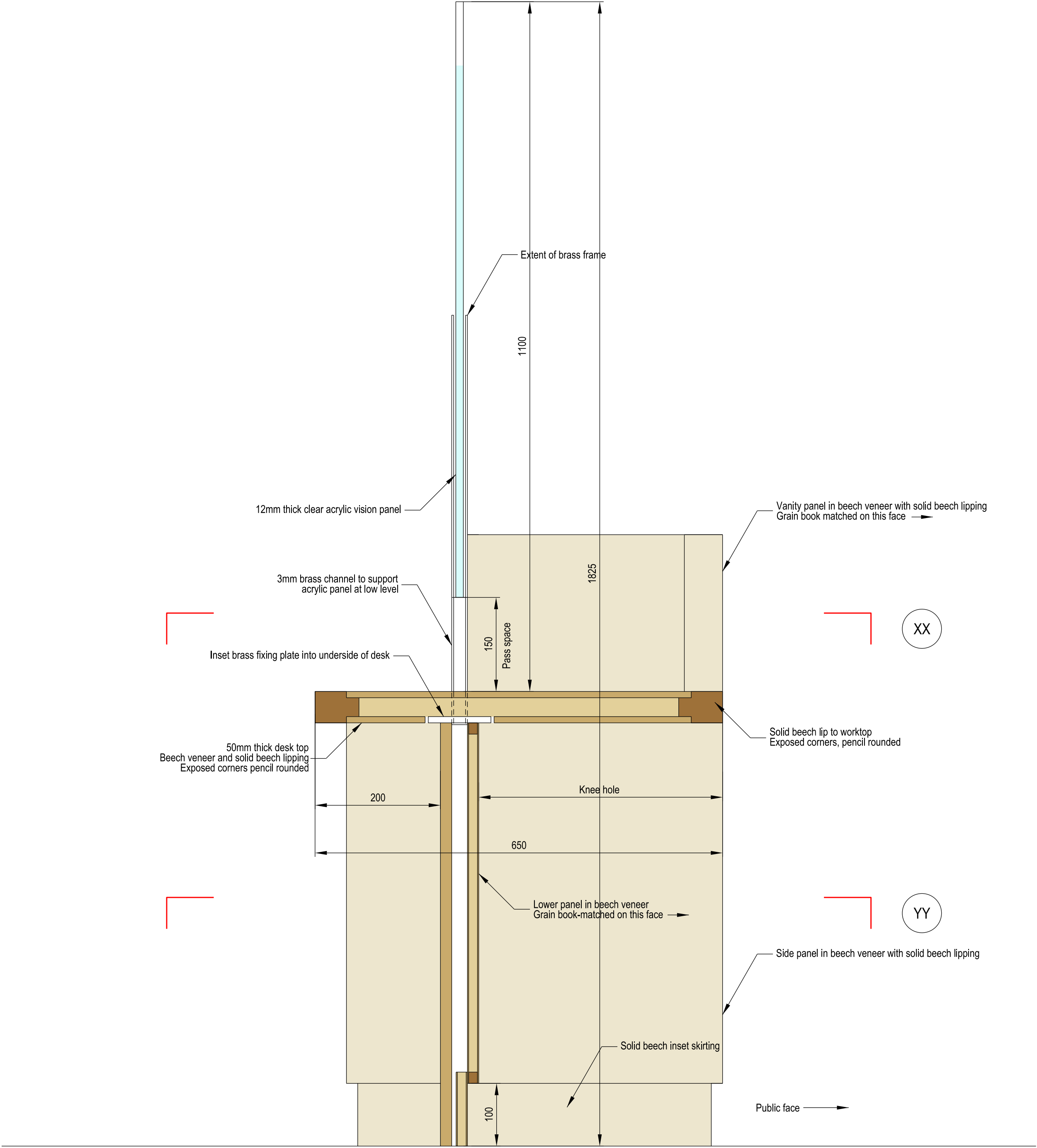
03 Proposed Section CC 1:5
