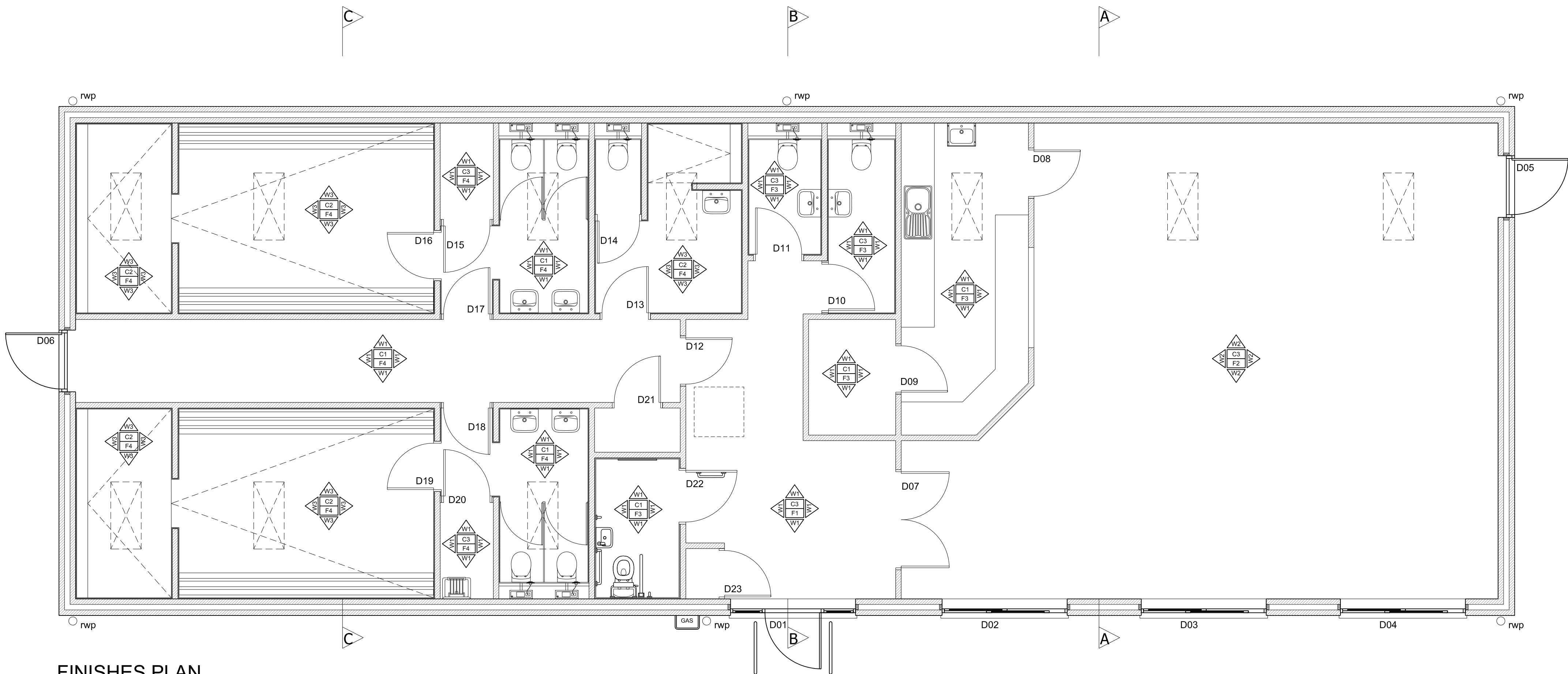
FINISHES PLAN
