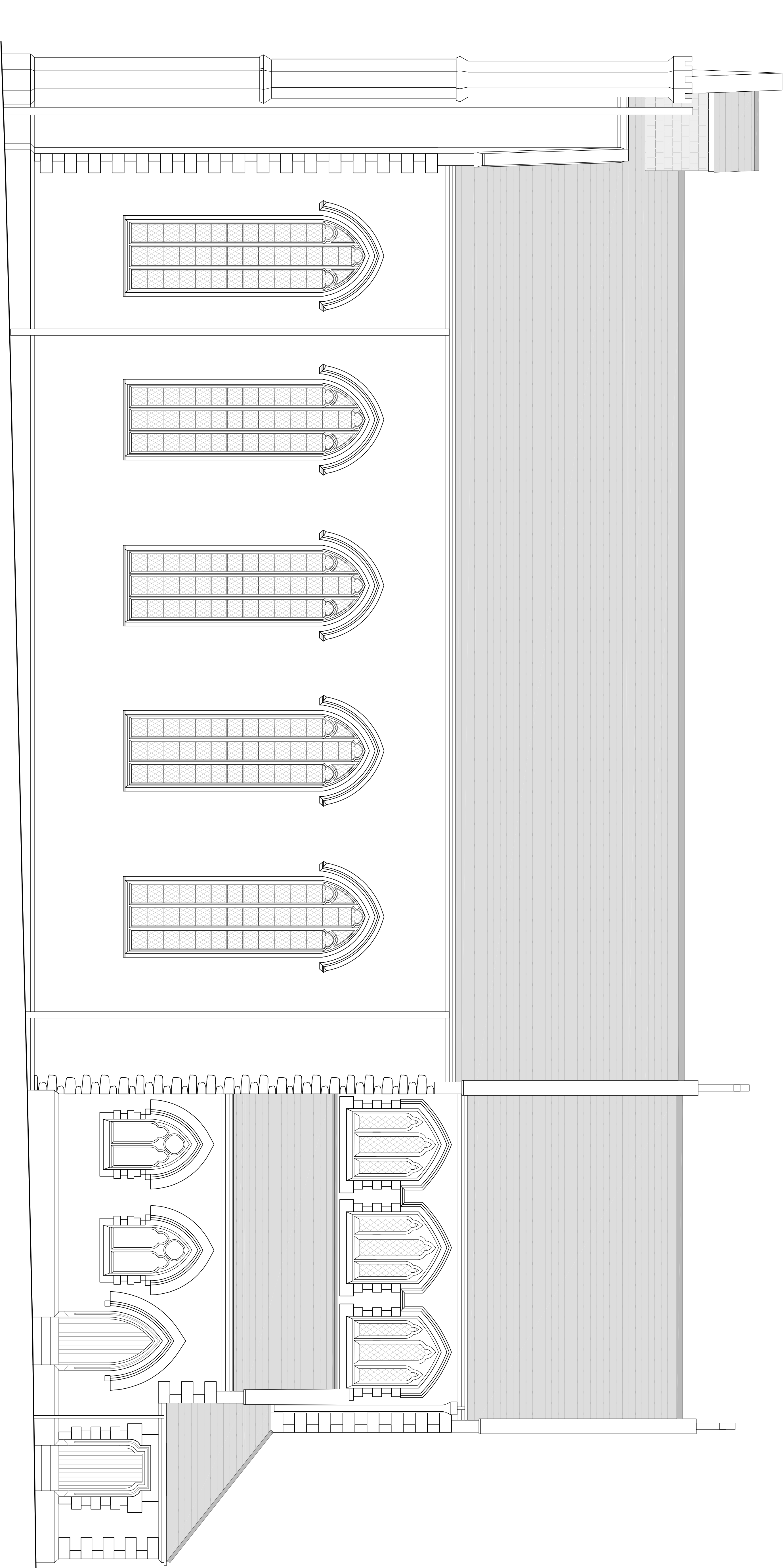
West Elevation
