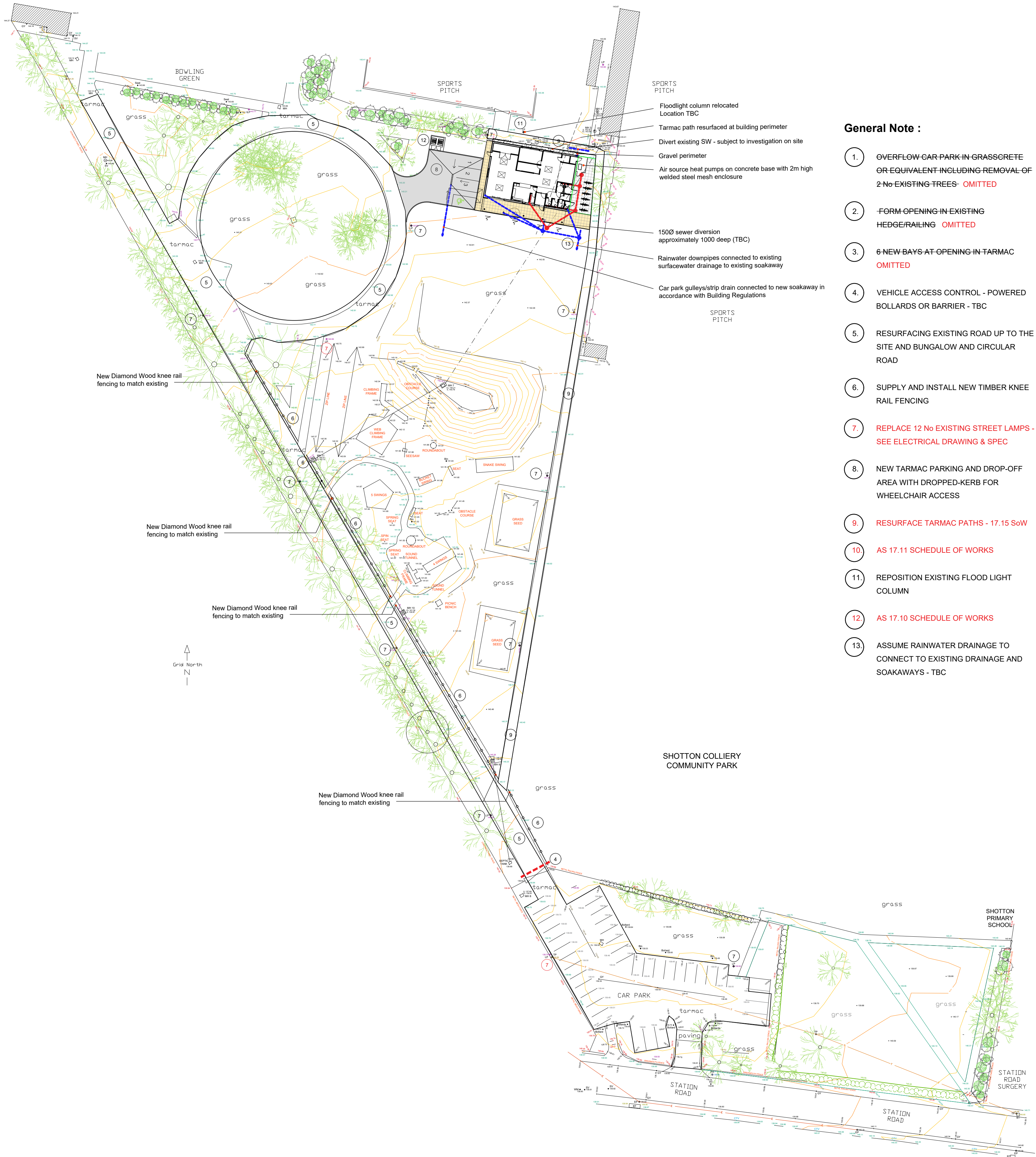
Proposed Site Plan & External Works 1 : 500 @A1
