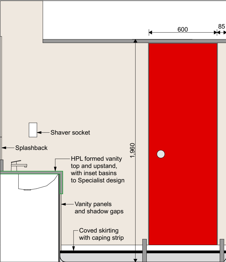
Cubicle Elevation 1:20
