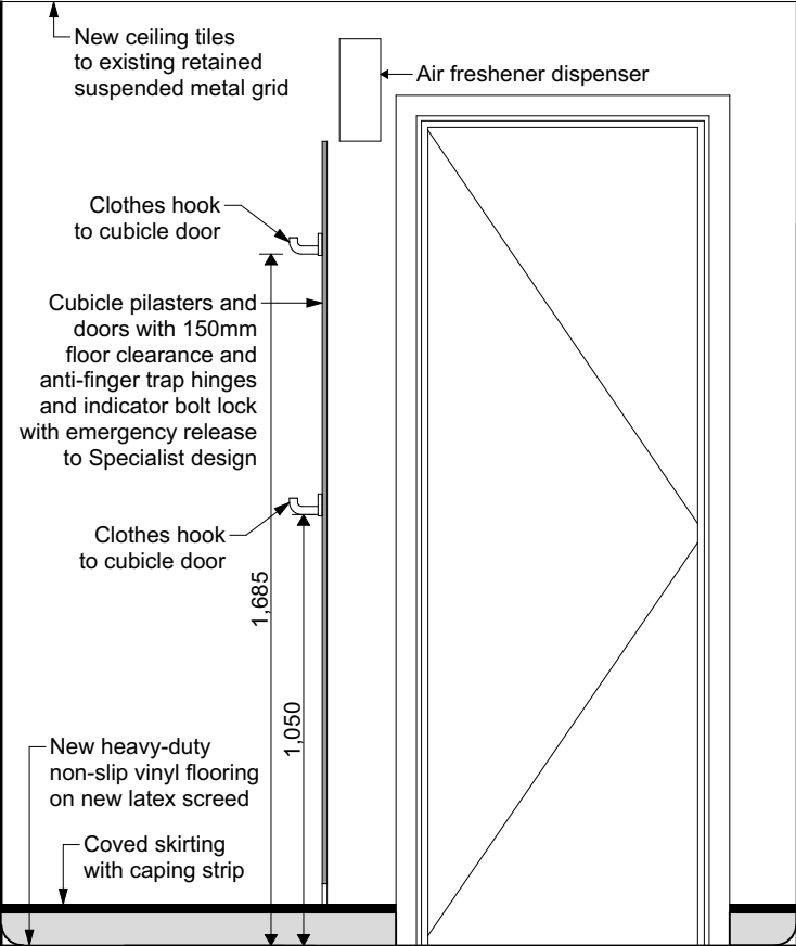
IE-02 05 Proposed Men WC 1:20
