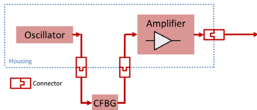
Figure 1: Principal building blocks of system. CFBG stands for chirped fibre Bragg grating which will be supplied by the customer.
