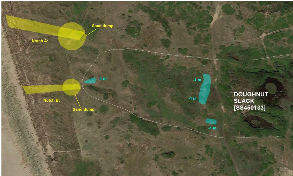
DOUGHNUT SLACK: NOTCHES & SEAWARD SLACK [Areas highlighted blue: elevated dune hummocks to be excavated by 1 metres in depth]
